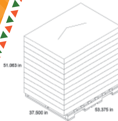
Pallet Layout
