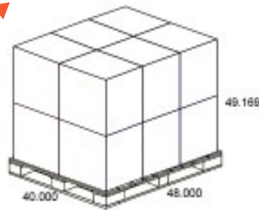
Pallet Layout
