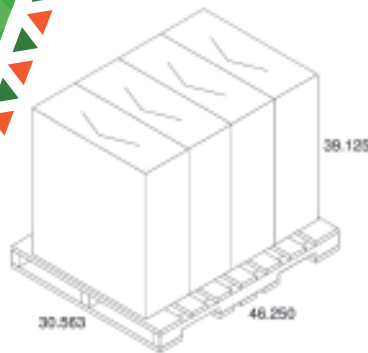
Pallet Layout
