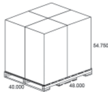
Pallet Layout
